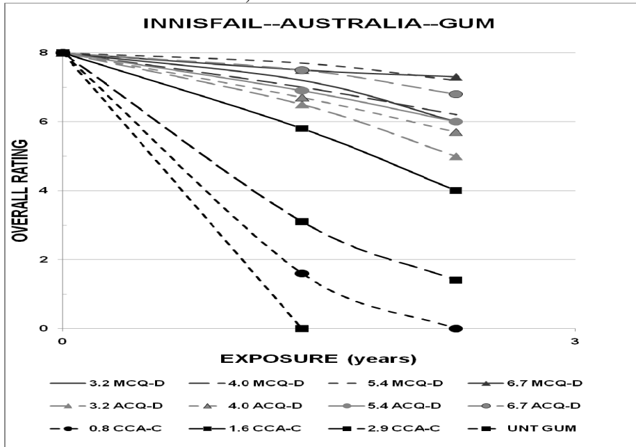
Figure 7. CSIRO Stake Test in Innisfail, Australia with Gum Stakes
