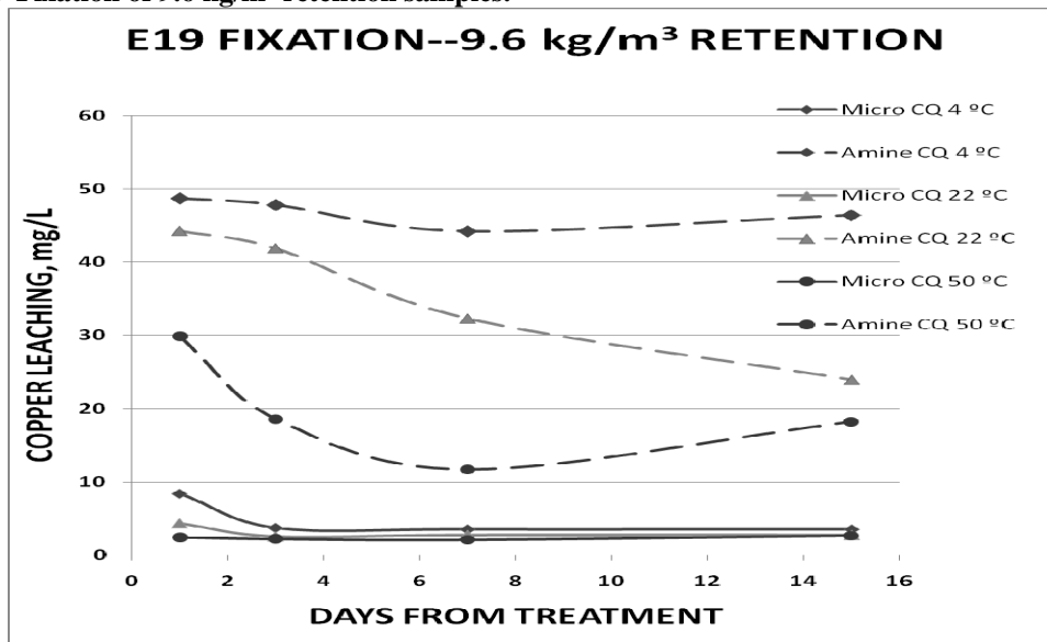
Figure 3. Fixation of 9.6 kg/m 3 retention samples.
