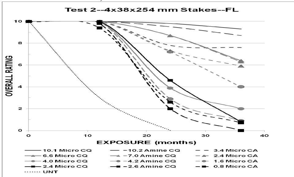
Figure 5. Stake Test 2 in Gainesville, FL with Fahlstrom Stakes
