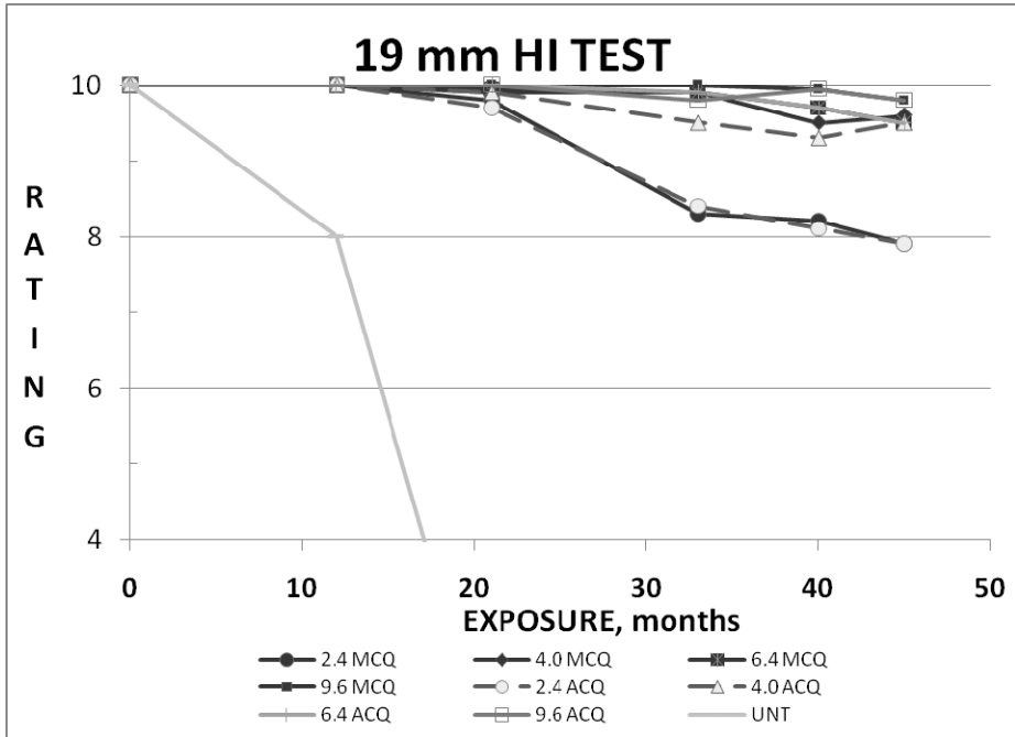
Figure 8. AWPA 19 mm Stake Test in Hawaii
