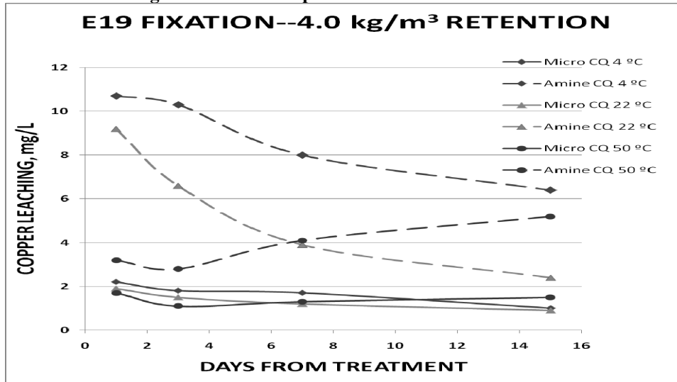
Figure 1. Fixation of 4.0 kg/m 3 retention samples.
