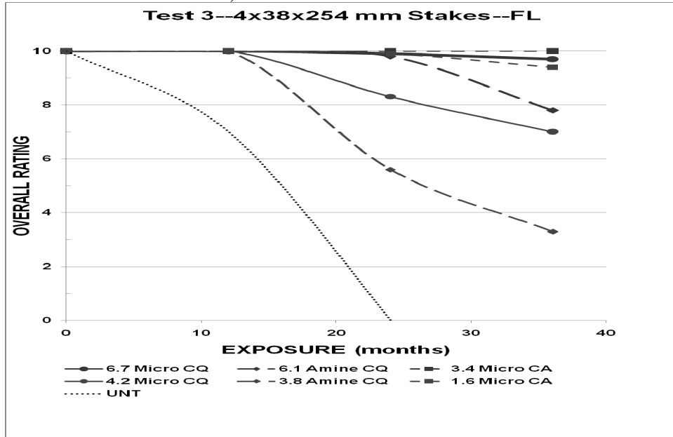
Figure 6. Stake Test 3 in Gainesville, FL with Fahlstrom Stakes
