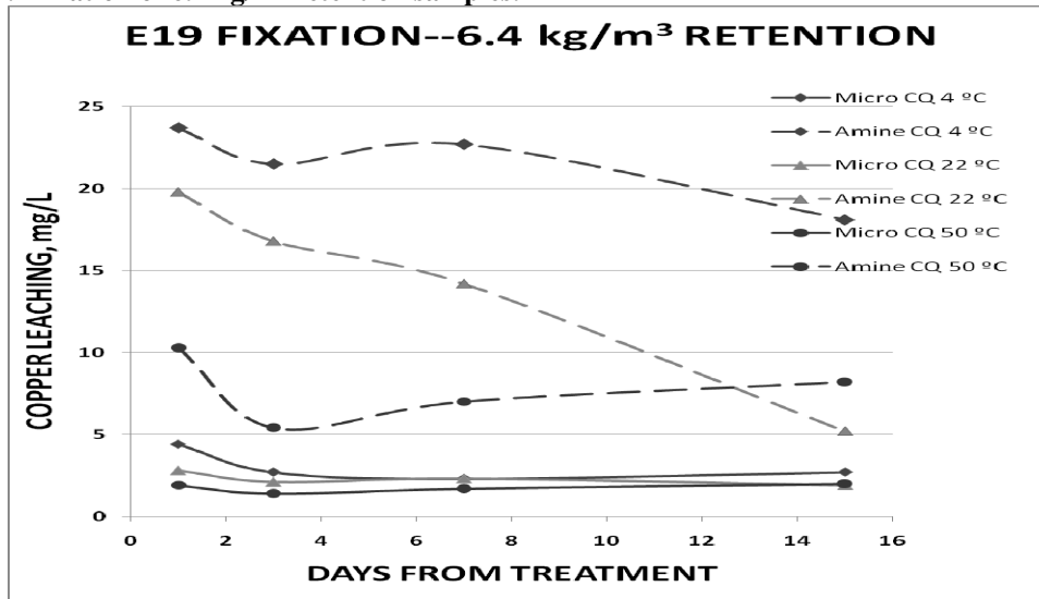
Figure 2. Fixation of 6.4 kg/m 3 retention samples.
