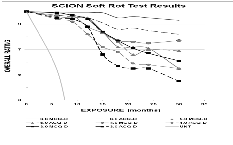
Figure 9. Soft Rot Test
