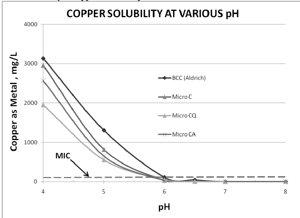
Figure 10. Solubility of copper at various pH.
